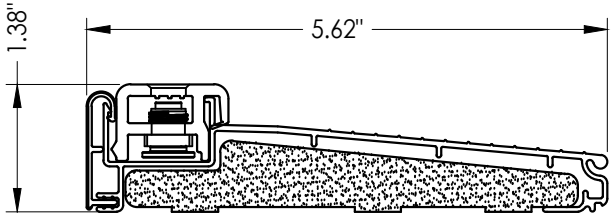
76 INSWING THRESHOLD
