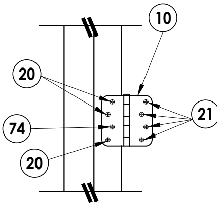
HINGE DETAIL 1
