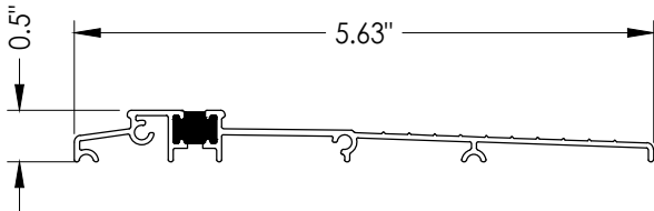
77 ADA THRESHOLD
