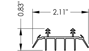
75 SWEEP
