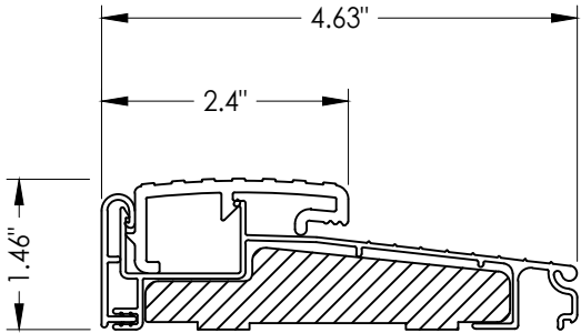
70 OUTSWING THRESHOLD
